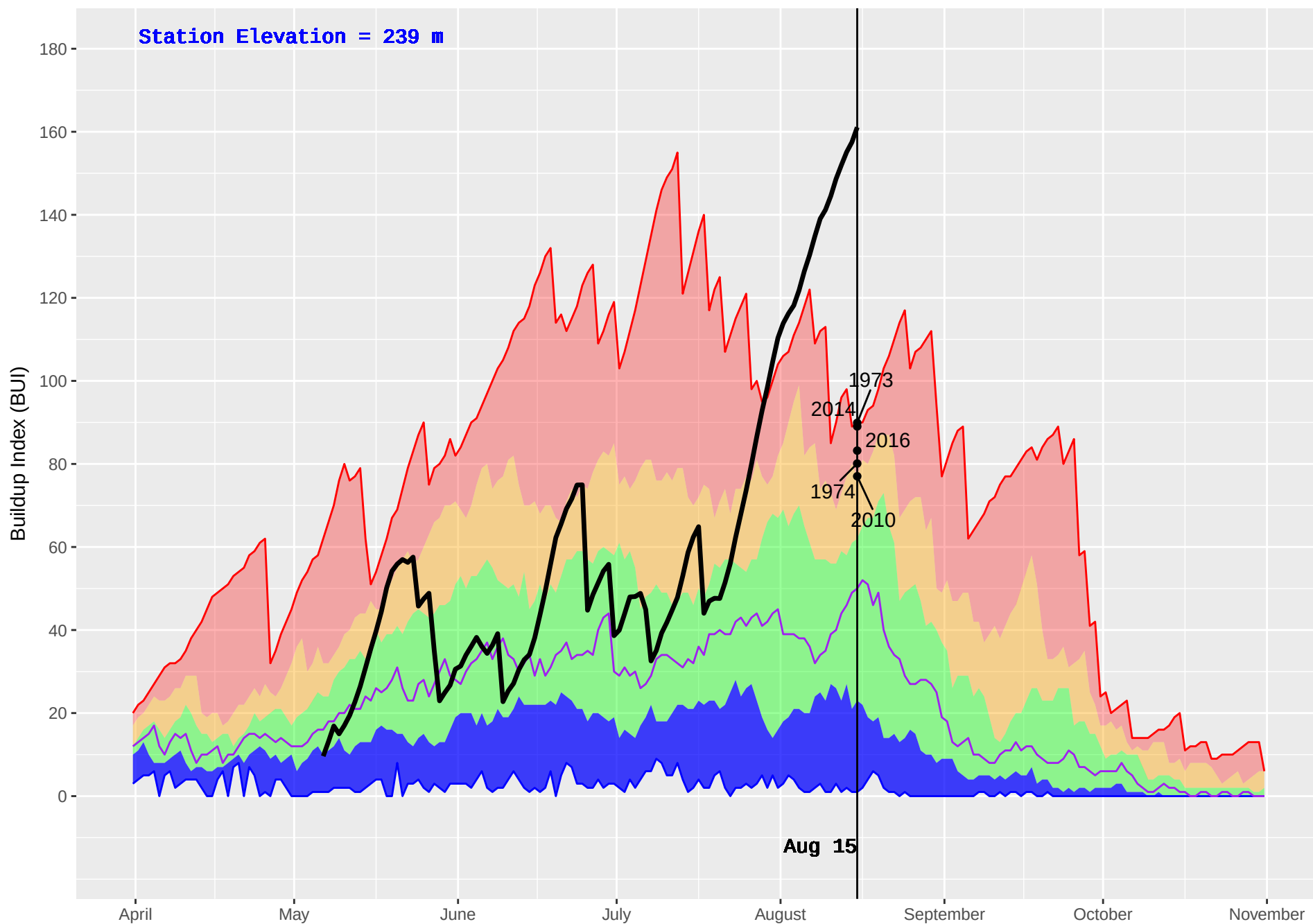
ROSSWOOD (105) : Historical (1970–2016) and Current (2018) Daily Buildup Index (BUI)
