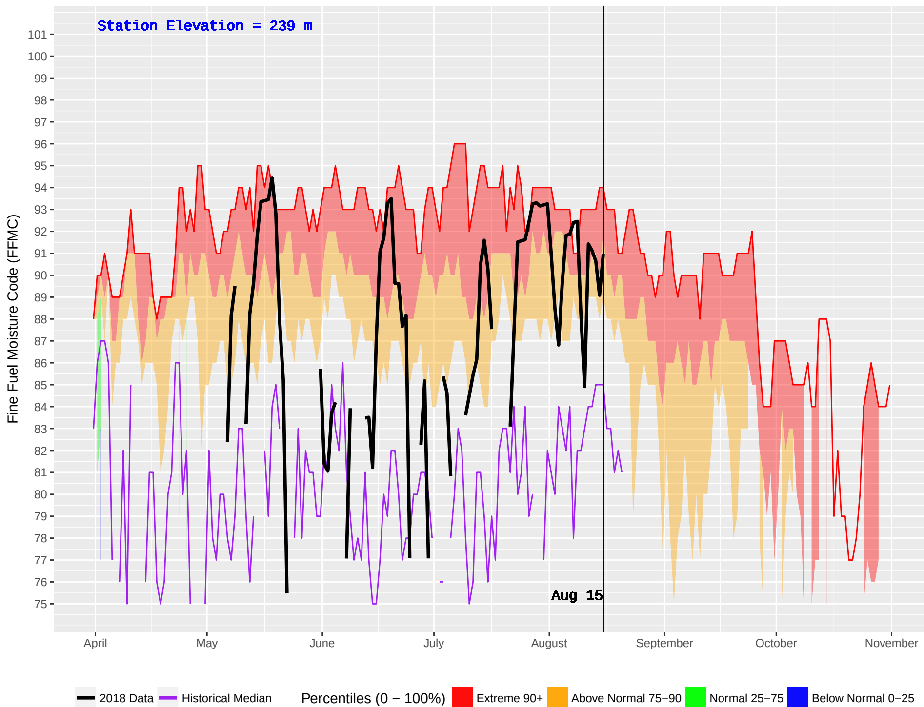
ROSSWOOD (105) : Historical (1970–2016) and Current (2018) Daily Fine Fuel Moisture Code (FFMC)
